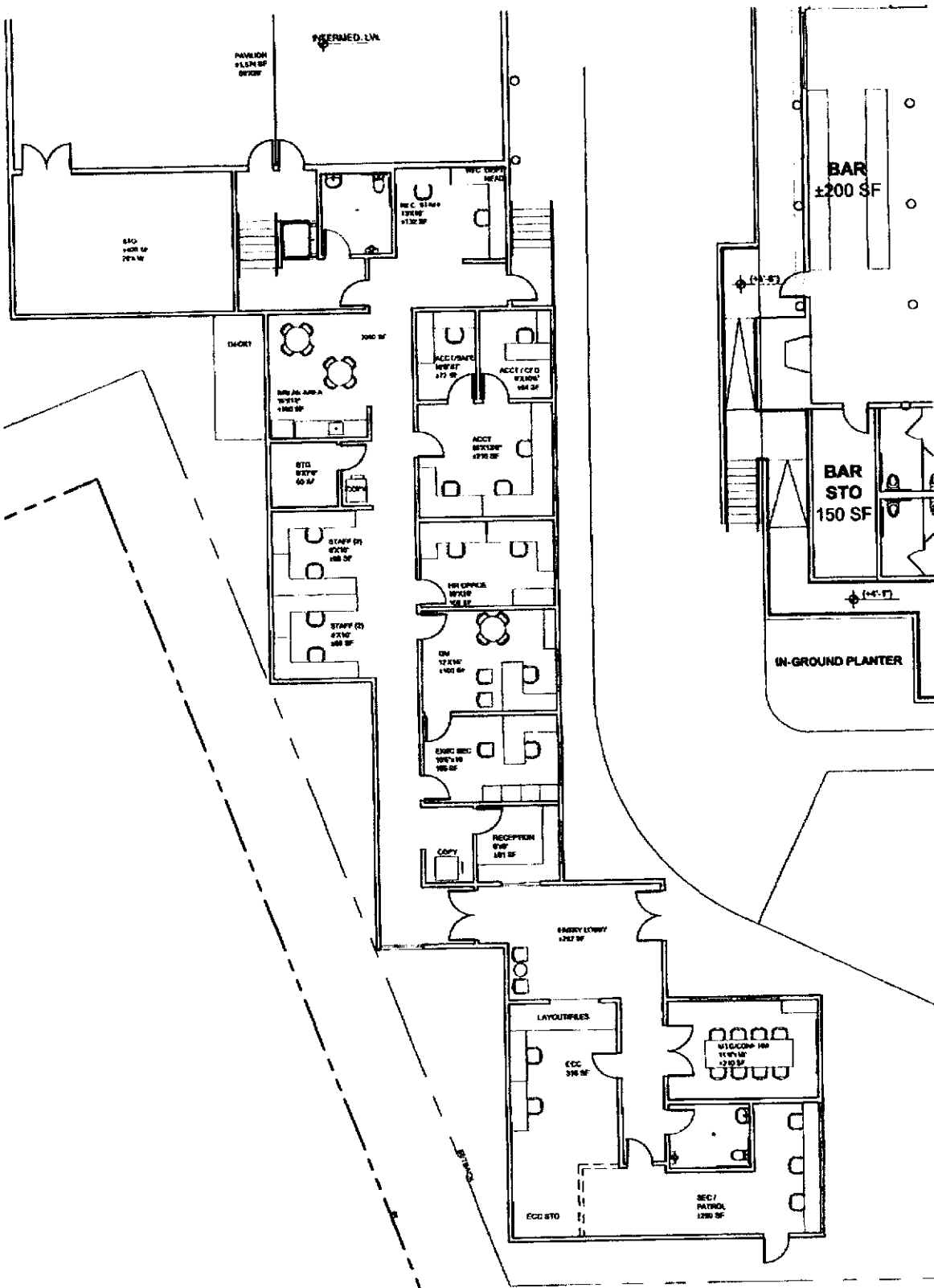
PMC ADMIN BUILDING CONCEPT PLAN 5-27-21 1/8" = 1'-0"
