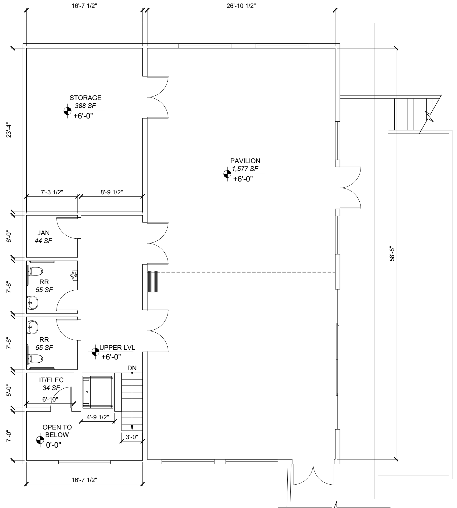
UPPER LVL FLOOR PLAN
